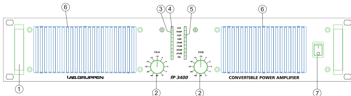
Figure 1: Front panel
